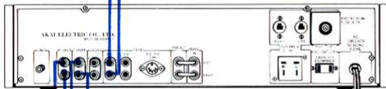
Stereo Amplifier
